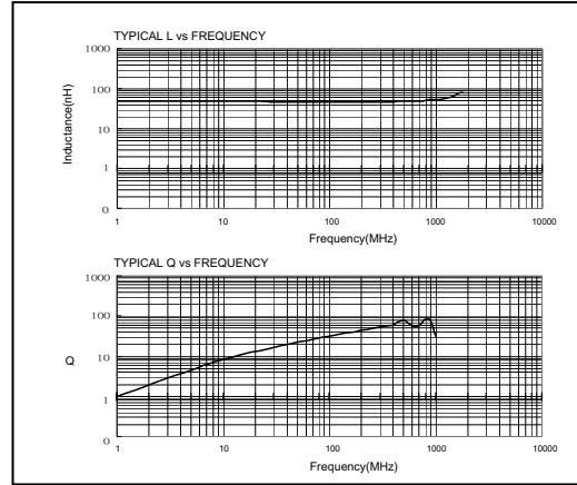
WTI-0603C-47NJ
