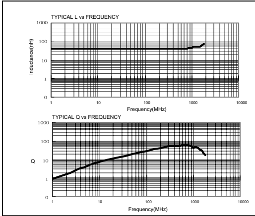
WTI-0603C-39NJ
